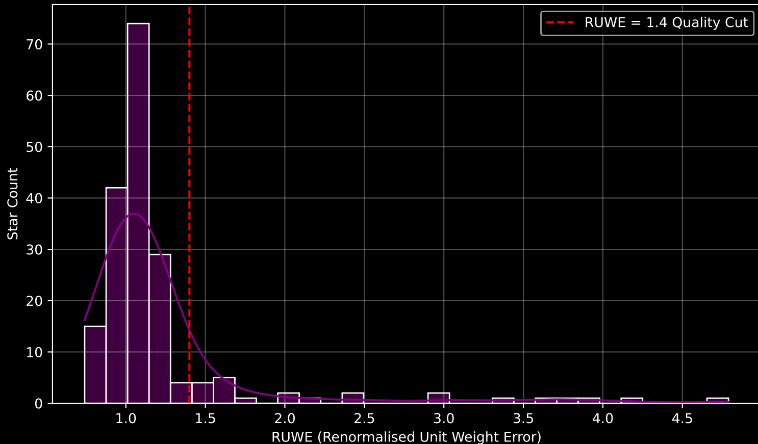
GAPOGEE DR17 Field [283-38-O_TESS] RUWE Distribution (n= 187)
