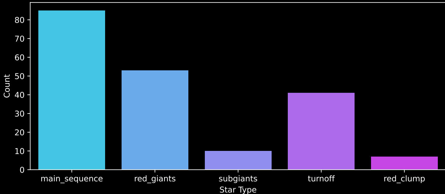
APOGEE DR17 Field: [283-38-O_TESS] Count plot of Star Type
